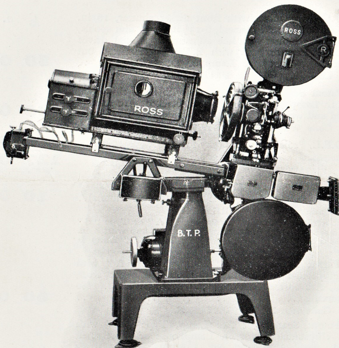
Ross F.C. Model, with Rear Flicker Shutter and Searchlight Arc Lamp, as adapted for use with B.T.P. Sound Equipment.
