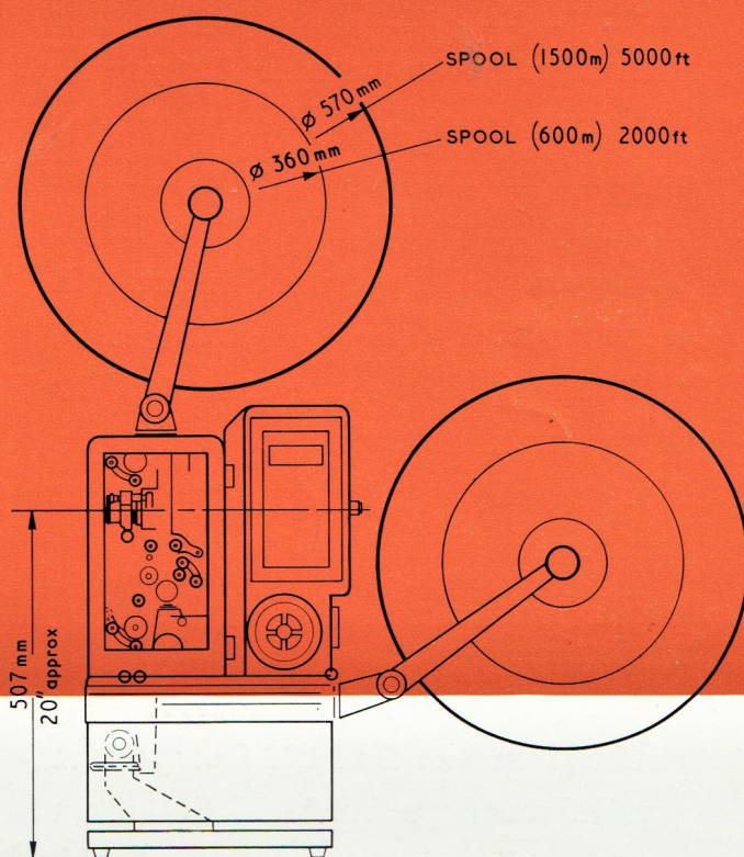
'LANGUEDOC' Mark II on short type stand
