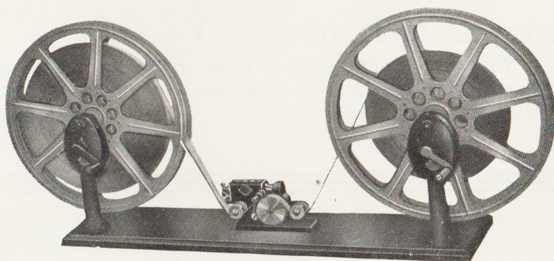
STANDARD MODEL (Illustrated with Film Measurer)
