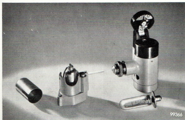
Sound-scanning unit, dismantled.
