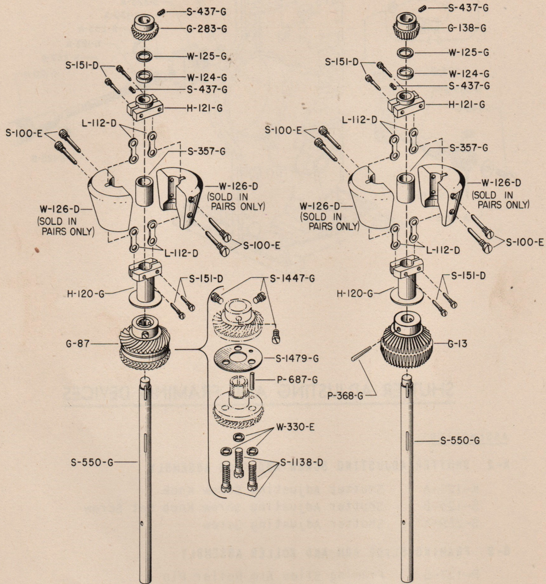
VERTICAL SHAFT (WITH SPIRAL BEVEL GEARS)
