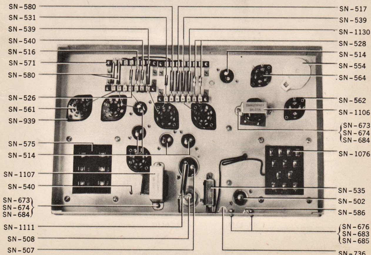
AM-1011 POWER AMPLIFIER
