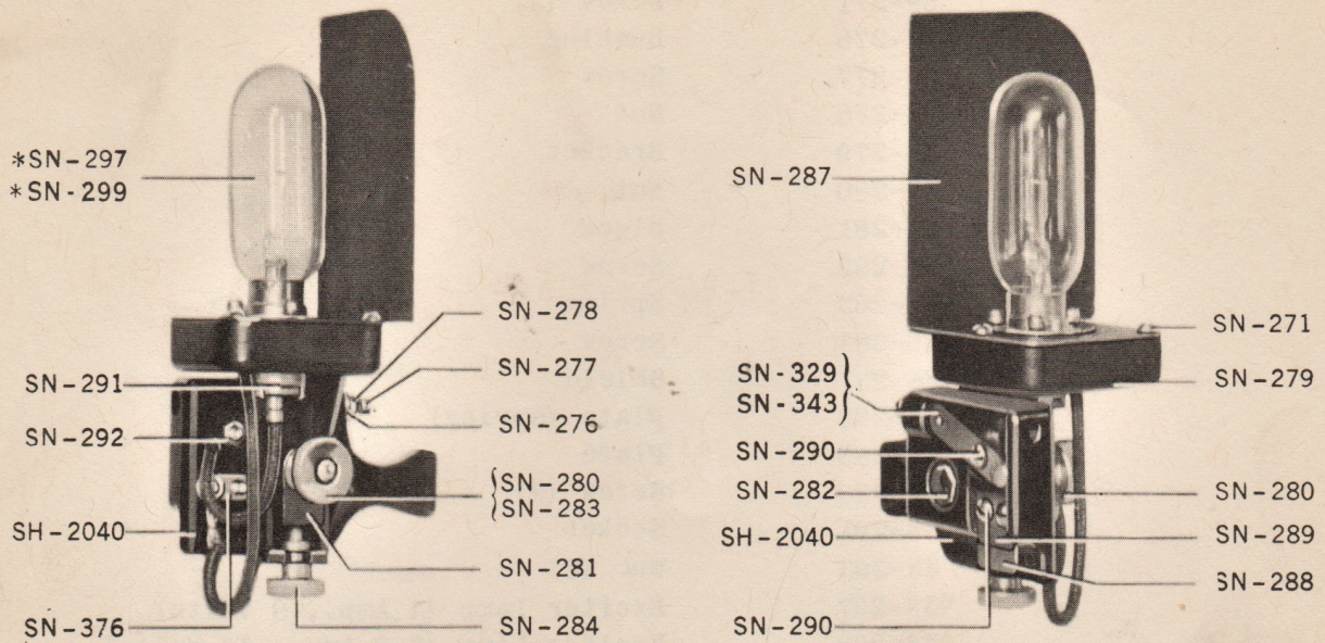
SH-2028 EXCITER LAMP BRACKET
