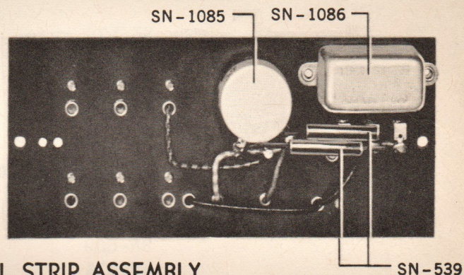
AM-2074 TERMIMAL STRIP ASSEMBLY
