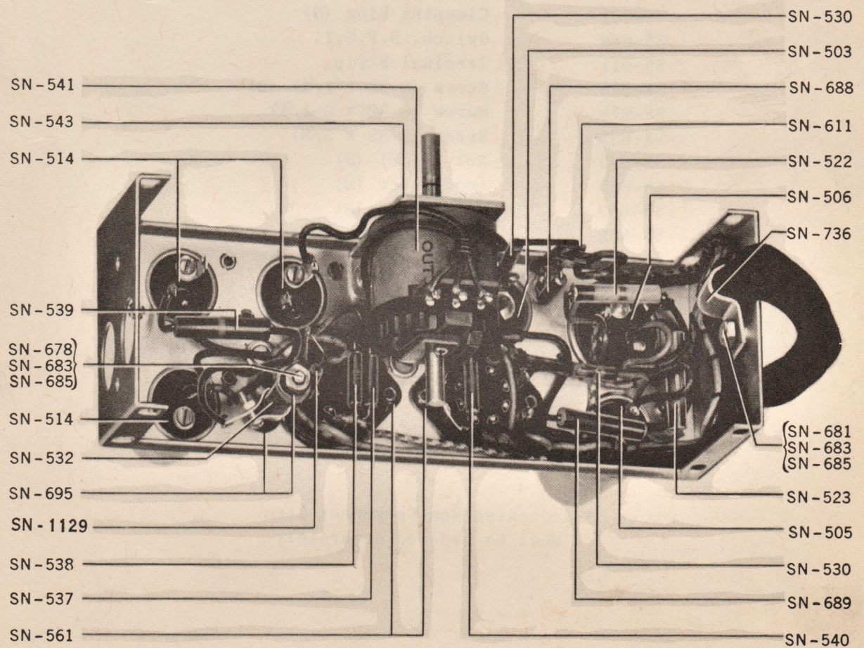
AM - 1000 VOLUME CONTROL AMPLIFIER
