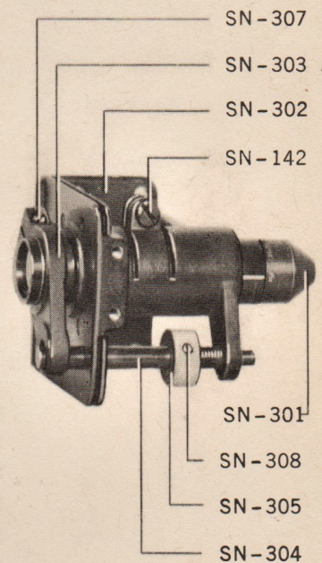
SH-2030 LENS ASSEMBLY
