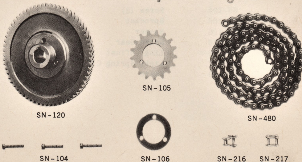
SH-2101 CHAIN TAKE-UP
