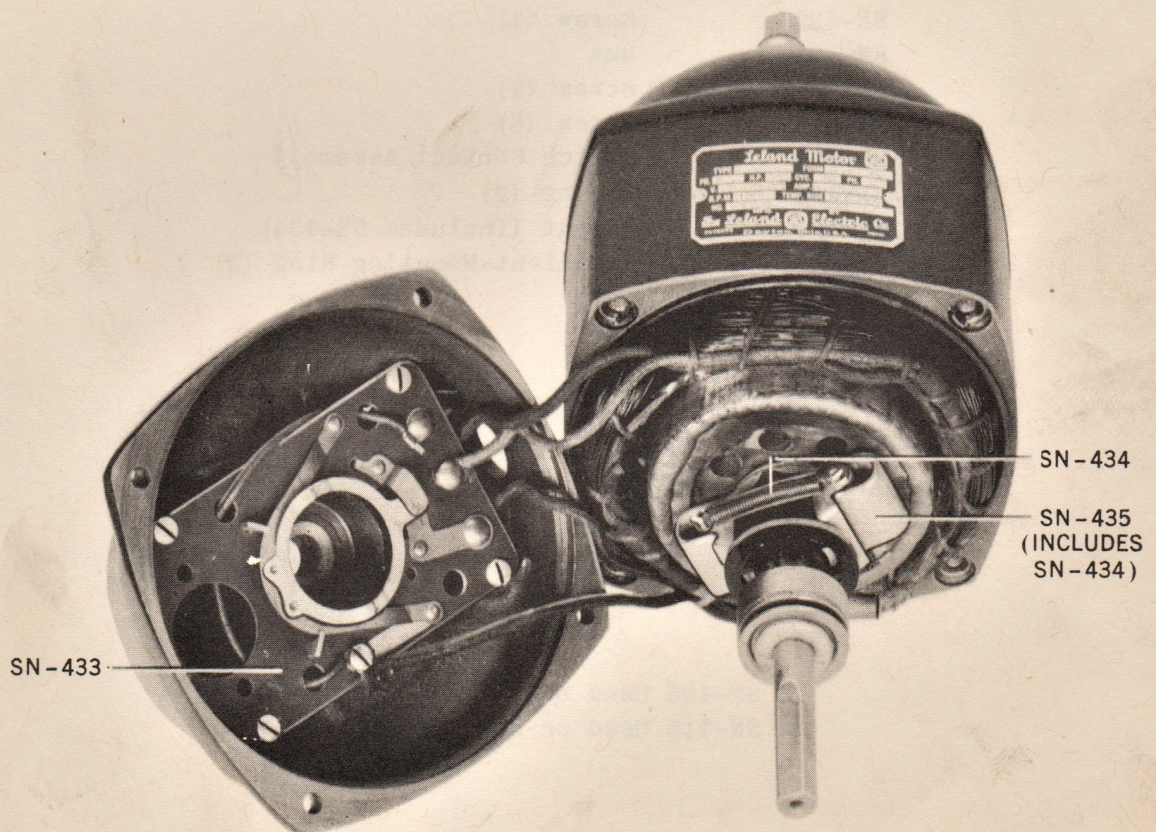
SH-2053 MOTOR ASSEMBLY - 60 CYCLE SH-2062 MOTOR ASSEMBLY - 50 CYCLE
