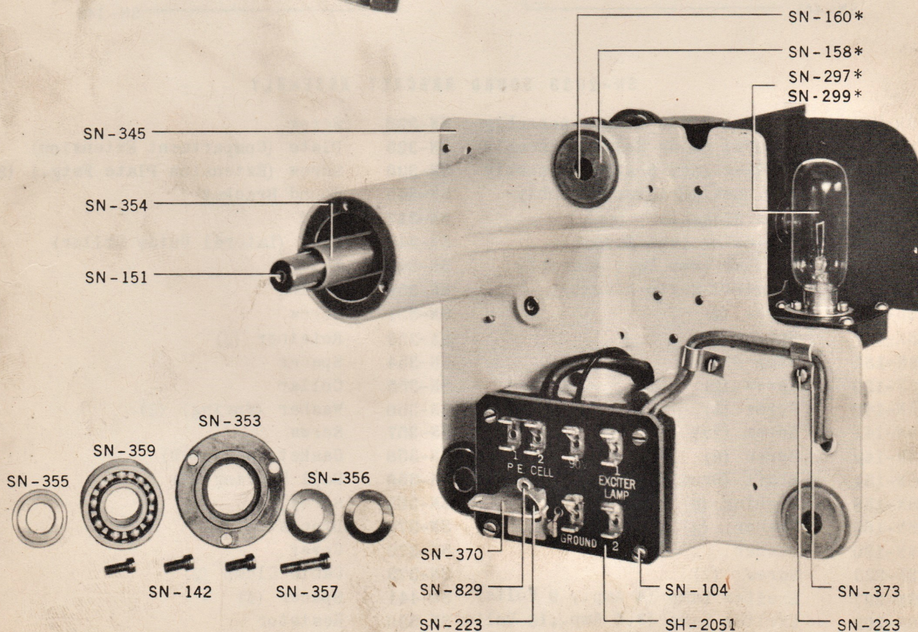
SH-2033 SOUND BRACKET ASSEMBLY
