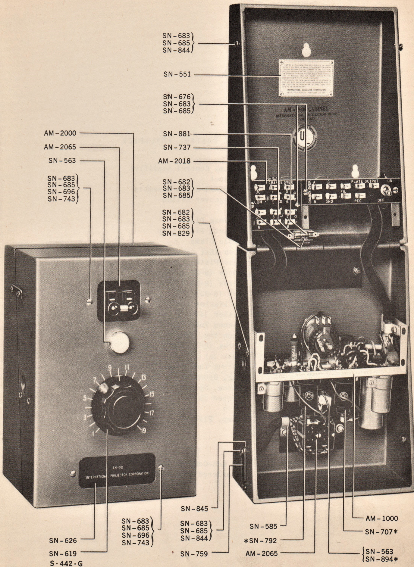
AM-101 VOLUME CONTROL AMPLIFIER
