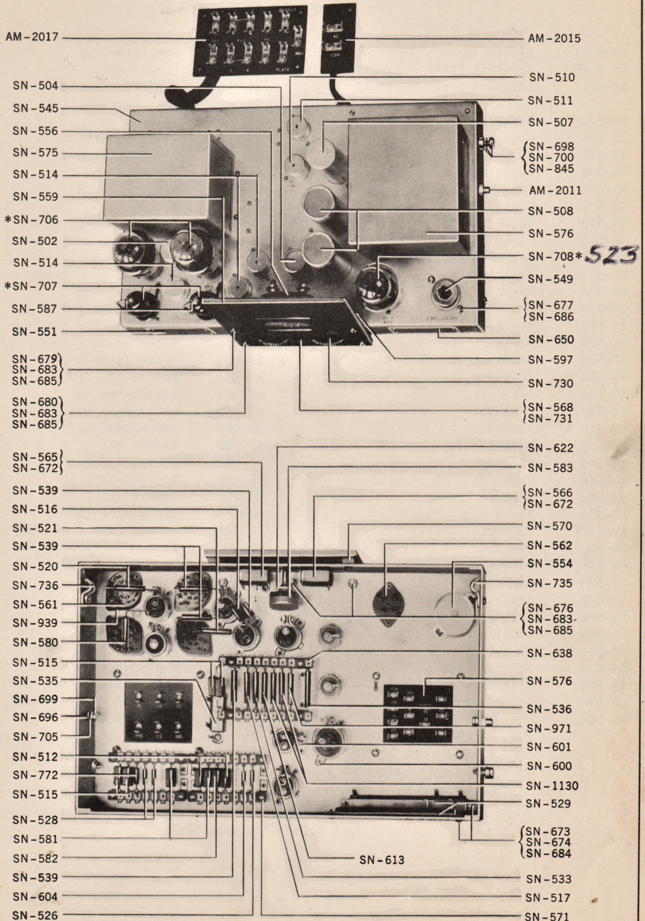
AM-1001 POWER AMPLIFIER
