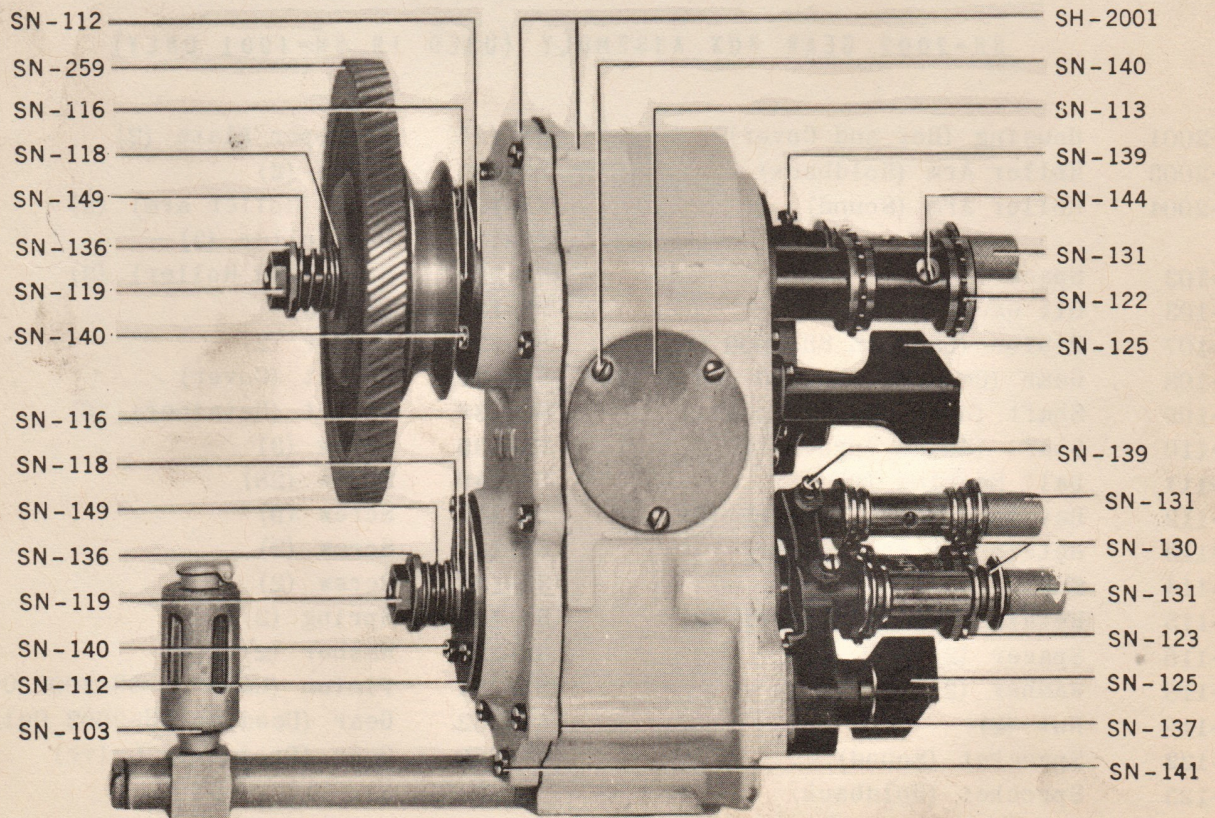
SH-2000 & SH-2002 GEAR BOX
