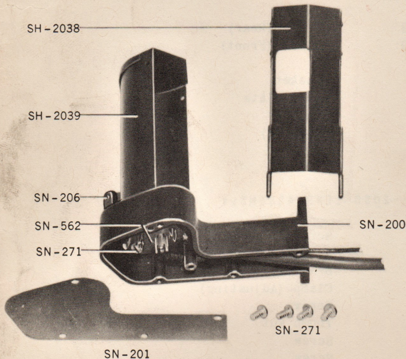
SH-2029 PHOTO-ELECTRIC CELL BRACKET
