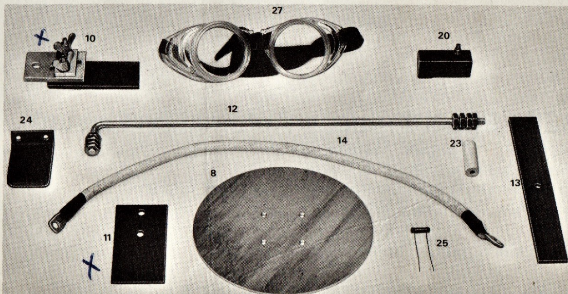
Spare parts for Xenon Lanterns.
