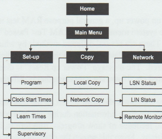
Figure 2.4: Menu structure for version 1.003 through 1.010.
