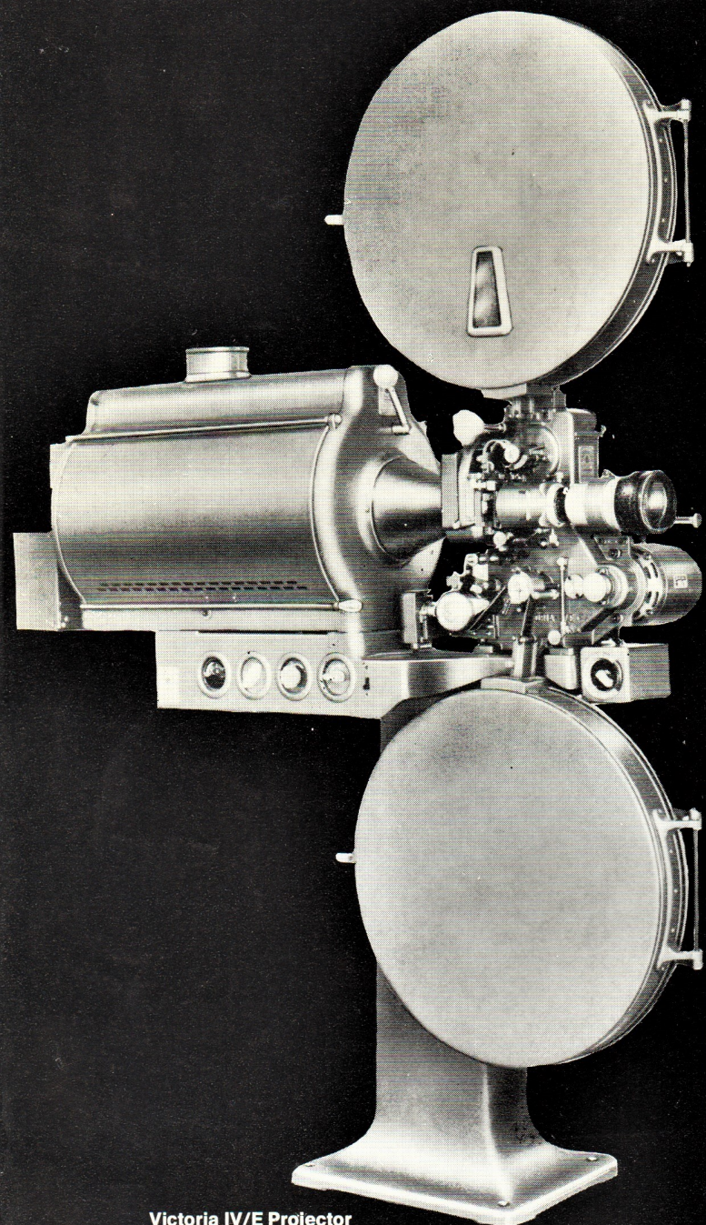
Victoria IV/E Projector with Zenith V Arc Lamp
