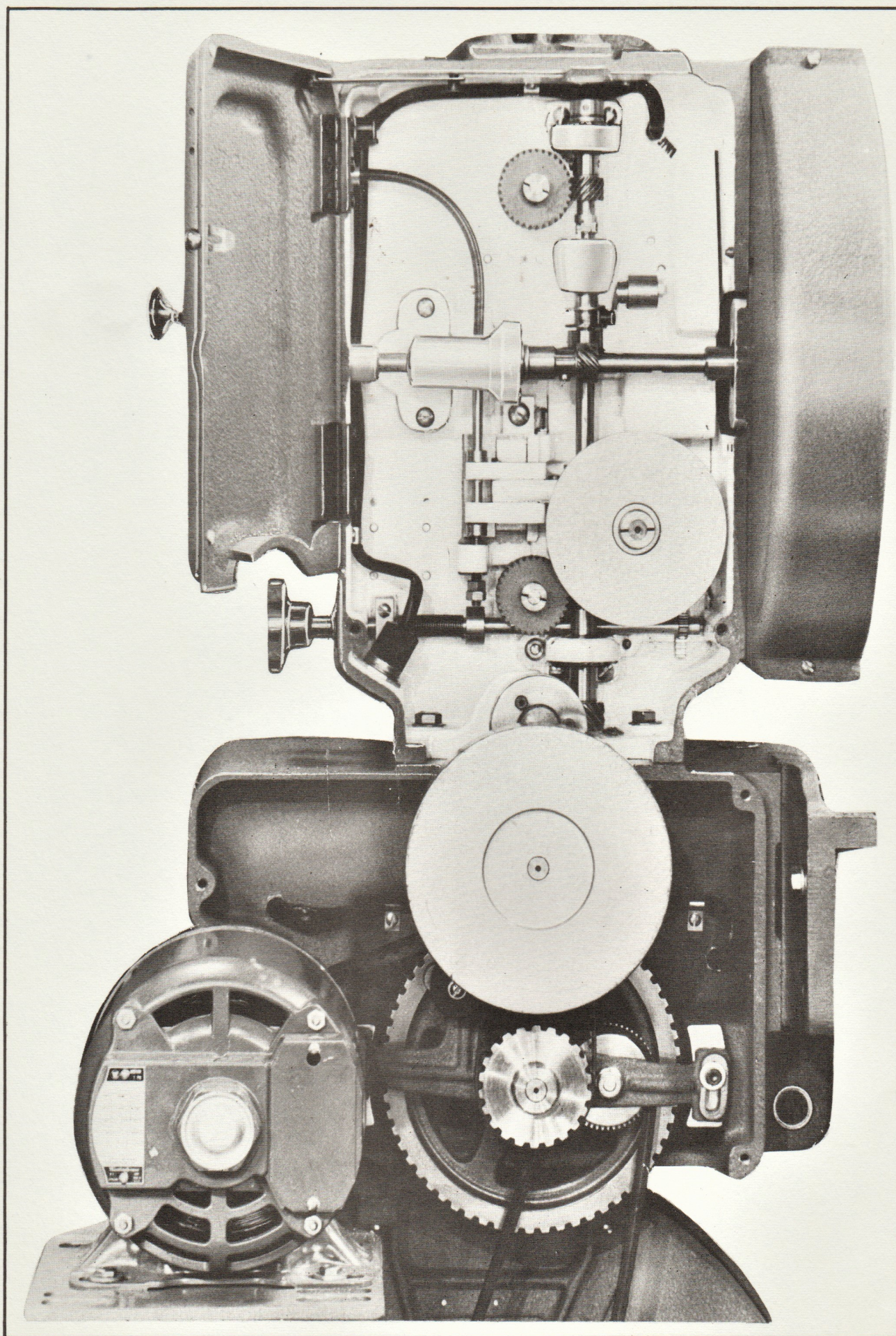
CENTURY PROJECTOR MECHANISM AND CENTURY SOUND REPRODUCER SINGLE SHUTTER-DRIVE SIDE
