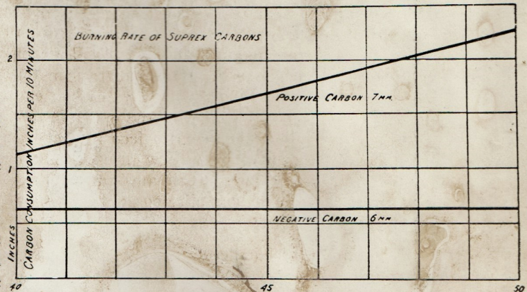
FIG. 1 Rate of consumption of Suprex carbons; 6-mm. negative and 7-mm. positive combination.
