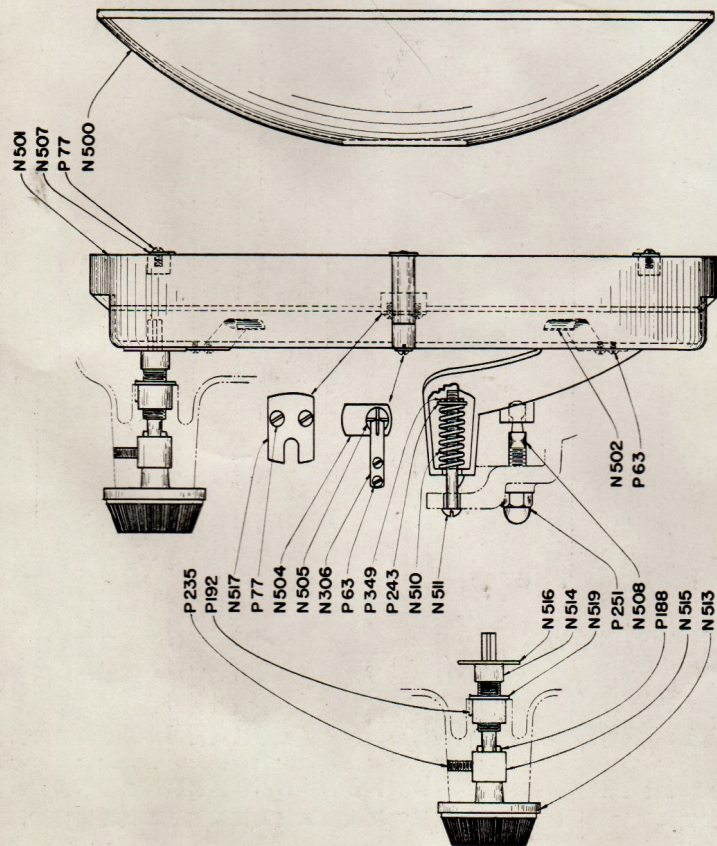
DIAGRAM No. 7 MIRROR UNIT
