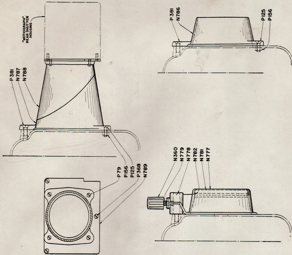
DIAGRAM No. 8 LAMPHOUSE FRONT CONES
