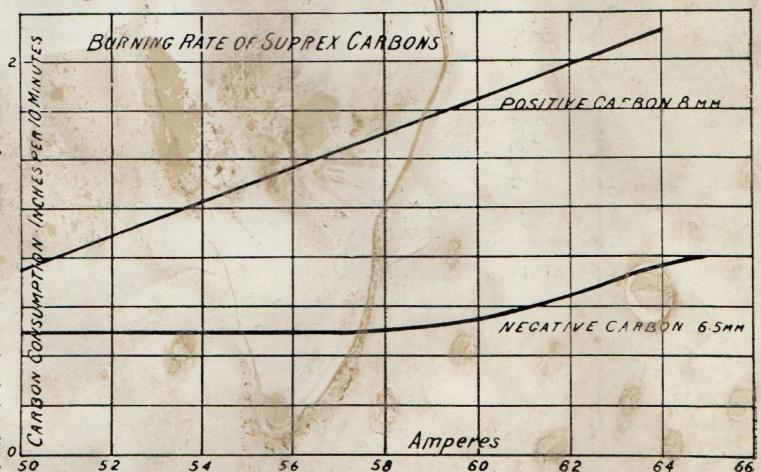
FIG. 2. Rate of consumption of Suprex carbons; 6.5-mm. negative and 8-mm. positive combination.
